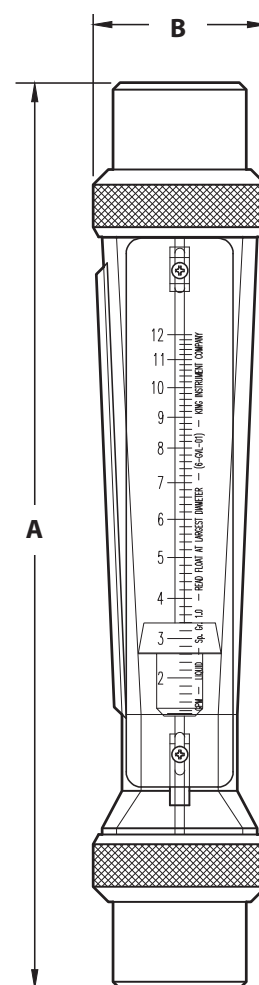
DIMENSION DIAGRAM
